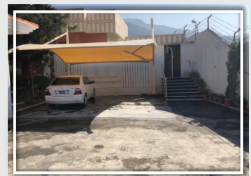
SWAT
